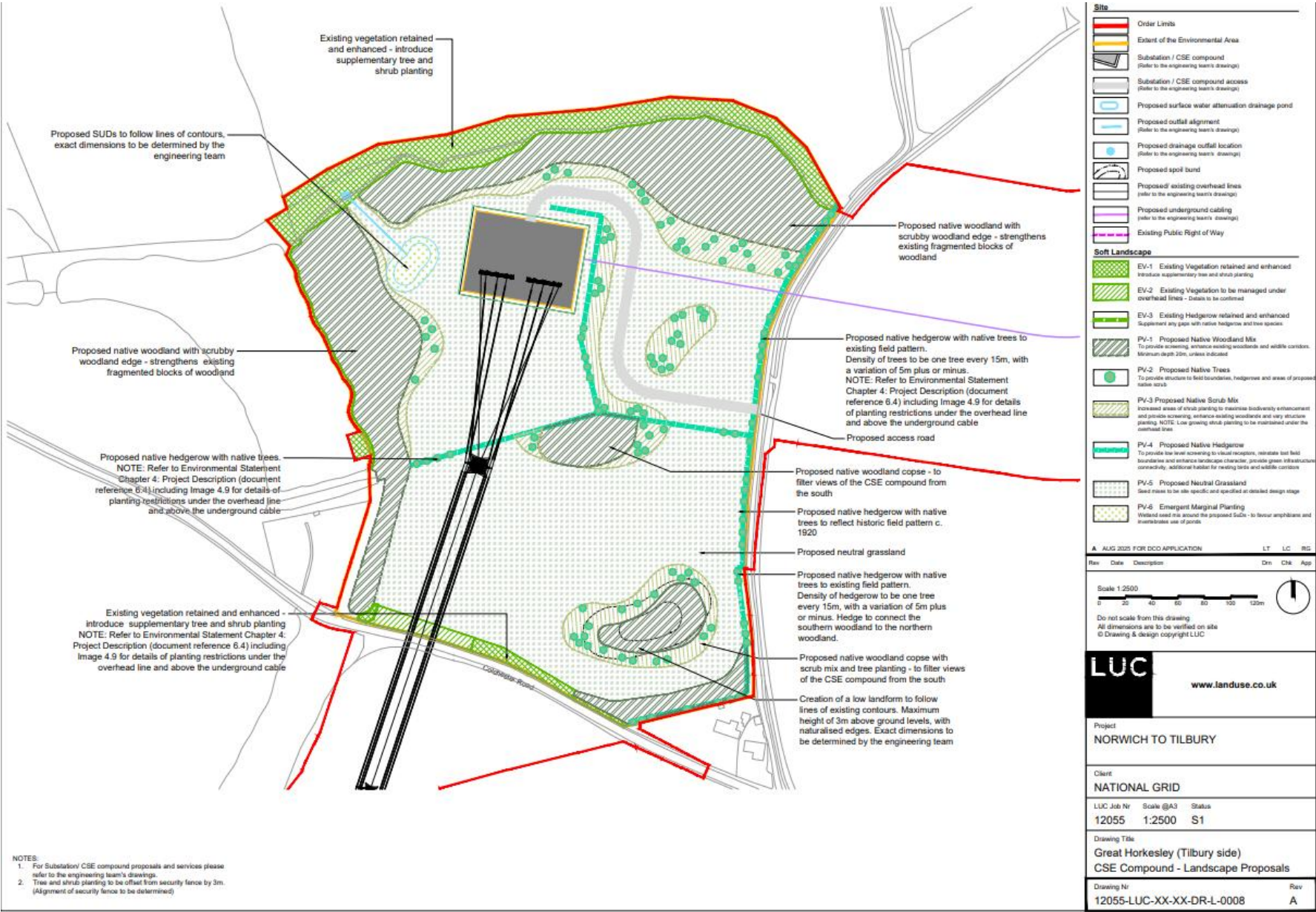
Image 1.4 Great Horkesley (Tilbury Side) Compound (Source: Appendix D of the Outline LEMP (Revision D))
