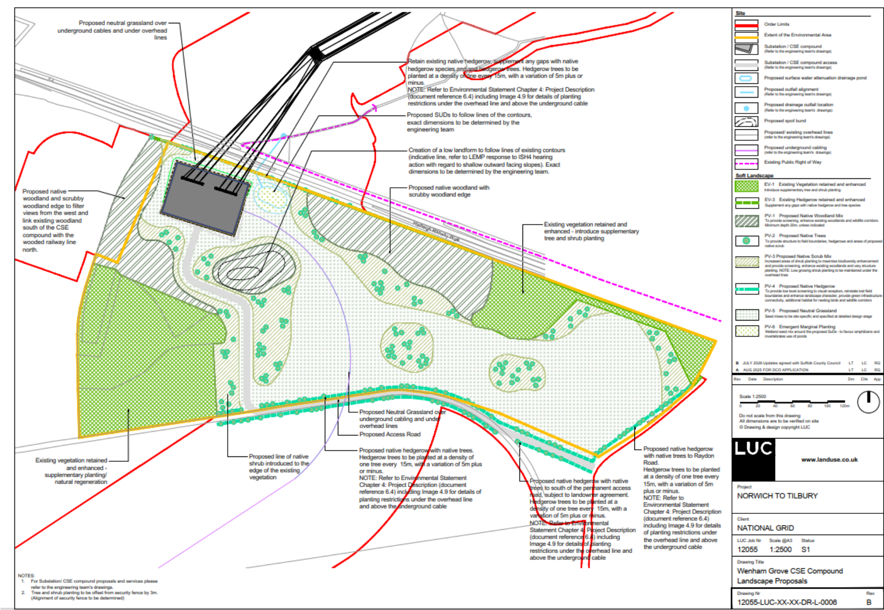
Image 1.2 Wenham Grove CSE Compound (Source: Appendix D of the Outline LEMP (Revision D))
